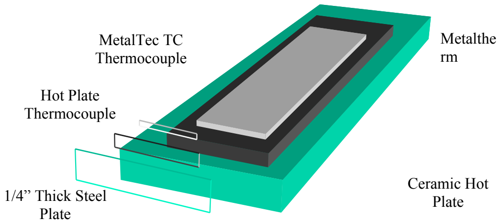
Graphic 1. Physical Contact Test Apparatus
